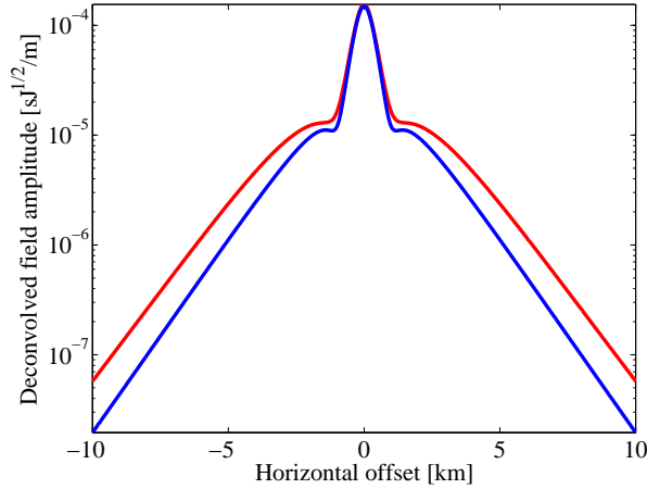
Figure 5. The reflection response \hat{R}_0^+(\mathbf{x}_A, \mathbf{x}, \omega) at f=0.25 Hz just below the sea bottom, obtained by interferometry-by-deconvolution. The result is independent of the water depth. The red and blue curves represent the situation with and without the reservoir layer, respectively.
