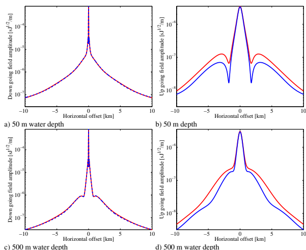
Figure 4. Decomposition of 2-D TM field at f=0.25 Hz just below the sea bottom. (a) Down going field and (b) up going field for a water depth h_w=50 m. (c) Down going field and (d) up going field for a water depth h_w=500 m. The red and blue curves represent the situation with and without the reservoir layer, respectively. In (a) and (c) the blue curves are hidden by the red curves.
