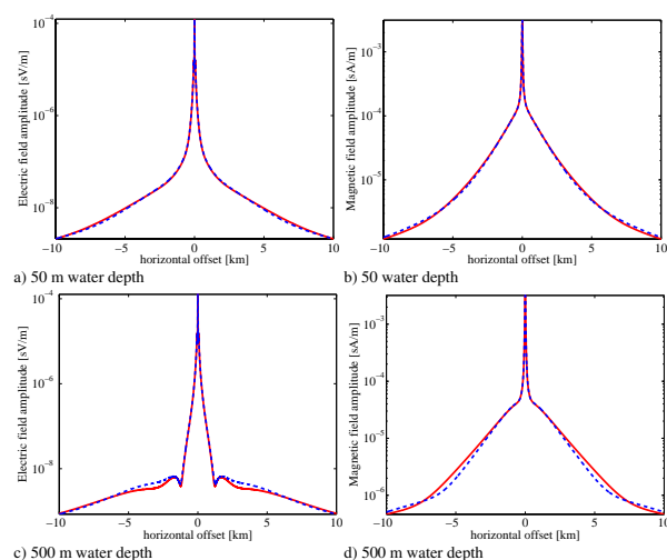
Figure 3. The electromagnetic field, at f=0.25 Hz, at the sea bottom. (a) The electric and (b) the magnetic field amplitudes for a water depth h_w=50 m. (c) The electric and (d) magnetic field amplitudes for a water depth of h_w=500 m. The red and blue curves represent the situation with and without the reservoir layer.
