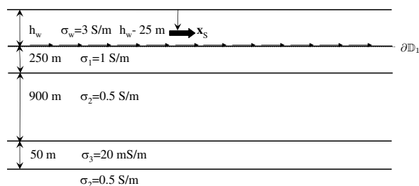
Figure 2. The configuration with a reservoir-type layer at 1150 m below the sea bottom and a water layer with variable thickness: h_w=50 m or h_w=500 m. The source is 25 m above the sea bottom and the receiver array is located at the sea bottom.
