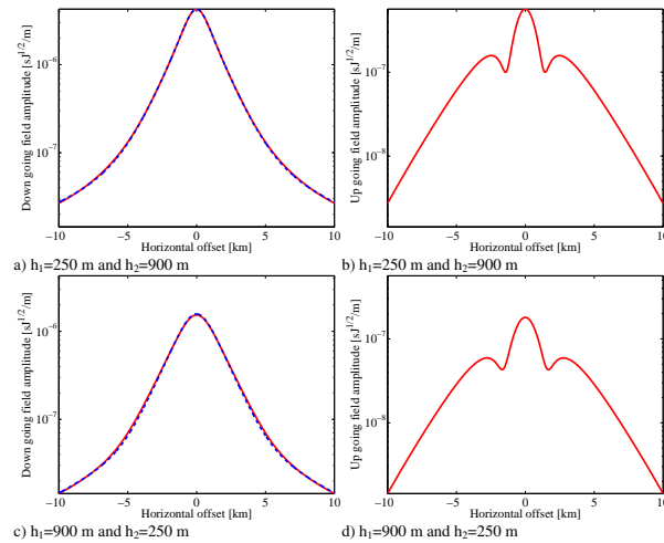
Figure 8. Decomposition of 2-D TM field at f=0.25 Hz in a horizontal borehole 200 m above the top of the reservoir layer. (a) Down going field and (b) up going field for h_1=250 m and h_2=900 m. (c) Down going field and (d) up going field for h_1=900 m and h_2=250 m. The red and blue curves represent the situation with and without the reservoir layer, respectively. In (a) and (c) the blue curves are hidden by the red curves. In (b) and (d) there are only red curves since in the situation without reservoir layer there are no up going fields.
