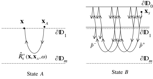
Figure 1. State A : the desired reflection response of the medium below \partial\mathbb{D}_1 , for the situation of a non-reflecting half-space above \partial\mathbb{D}_1 . State B : the actual response of the real earth, bounded by a free surface at \partial\mathbb{D}_0 . The medium parameters exhibit dissipation, are 3-D inhomogeneous functions of position, and below \partial\mathbb{D}_1 they are the same in both states.
