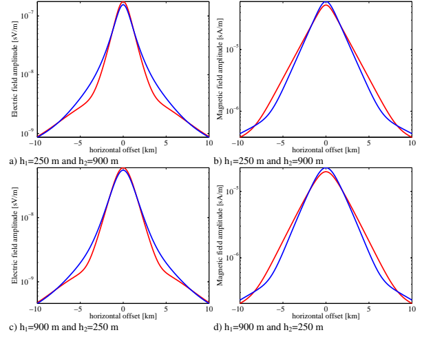
Figure 7. Electric and magnetic field amplitudes, at f=0.25 Hz, in a horizontal borehole 200 m above the top of the reservoir layer. (a) The electric field and (b) the magnetic field for h_1=250 m and h_2=900 m. (c) The electric field and (d) the magnetic field for h_1=900 m and h_2=250 m. The red and blue curves represent the situation with and without the reservoir layer.
