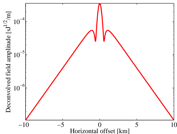
Figure 9. The reflection response \hat{R}_0^+(\mathbf{x}_A, \mathbf{x}, \omega) at f=0.25 Hz in a horizontal borehole 200 m above the top of the reservoir layer, obtained by interferometry-by-deconvolution. The result is independent of the overburden.
