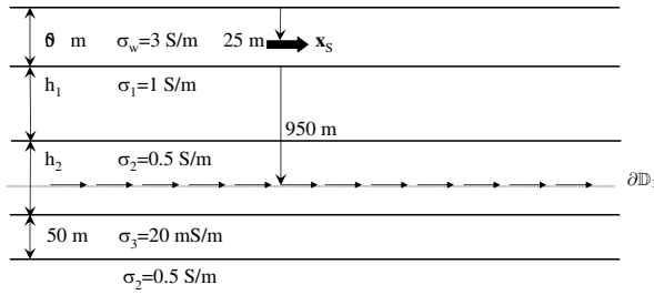
Figure 6. The configuration with a reservoir-type layer at 1150 m below the sea bottom and a water layer with a fixed thickness of 50 m. The source is 25 m above the sea bottom and the receiver array is located in a horizontal borehole 950 m below the sea bottom and 200 m above the top of the reservoir layer. The Earth layers have variable thicknesses: h_1=250 m and h_2=900 m, or h_1=900 m and h_2=250 m.
